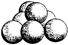
Protons (red marbles) have positive electric charge
