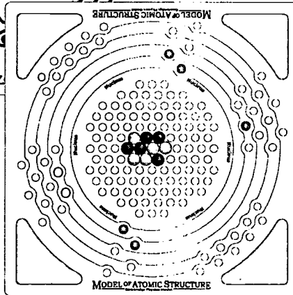
MODEL OF ATOMIC STRUCTURE
