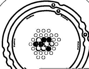
MODEL OF ATOMIC STRUCTURE
